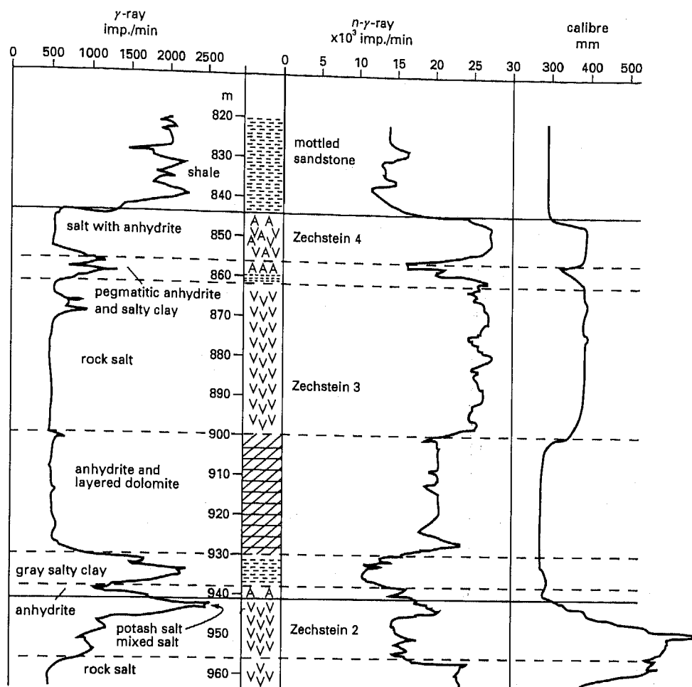
Figure 2. Radiometric logging graphs from the Zechstein subdivision of Thuringia (from ref. 13).
